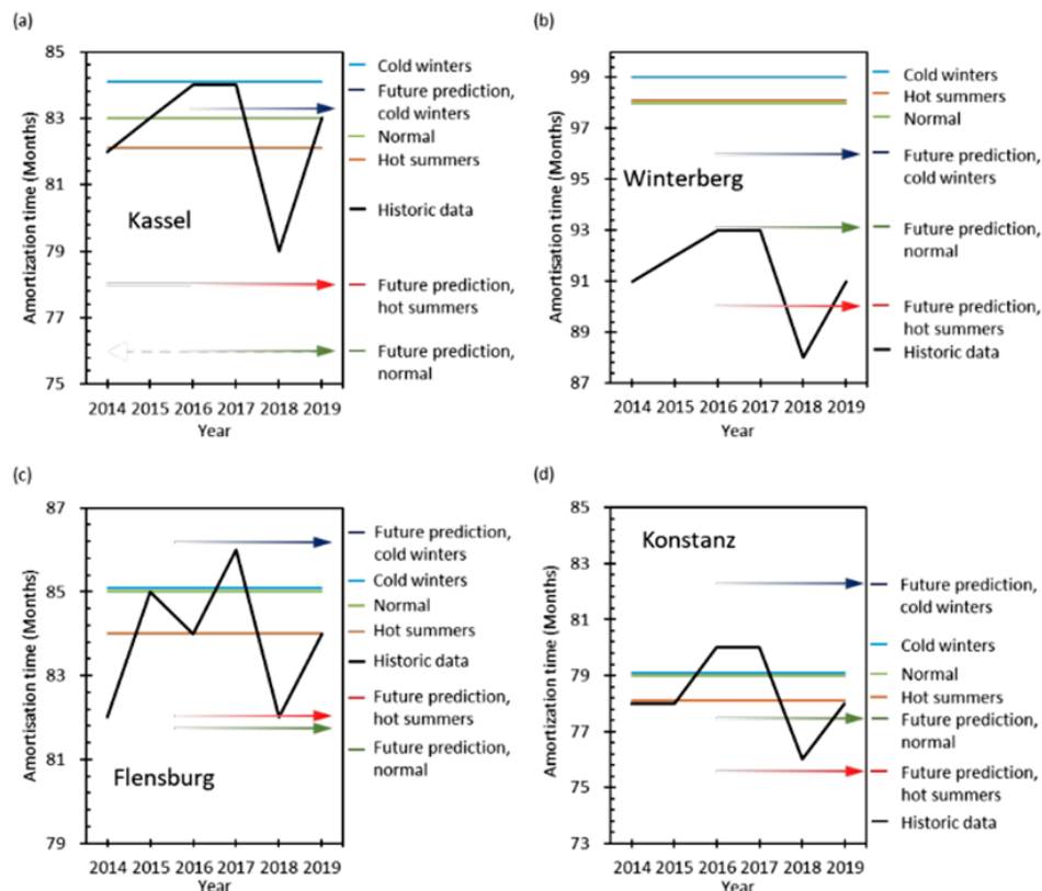
Figure 19. Illustration of amortization time considering the historic data from 2014 to 2019, mean actual TRY generated from previous observation – termed as “normal”, winter and summer dominant actual TRY generated from previous observation – termed as “cold winters” and “hot summers”, and future predicted TRY created by the assumption based on previous observations – termed as “future prediction”, represented by arrows facing right towards the future for (a) Kassel, (b) Winterberg, (c) Flensburg and (d) Konstanz.
