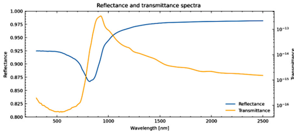
Figure 8. Simulated reflectance and transmittance spectra of the modelled metallic multilayer system. Modified figure from Ref. [28] .
