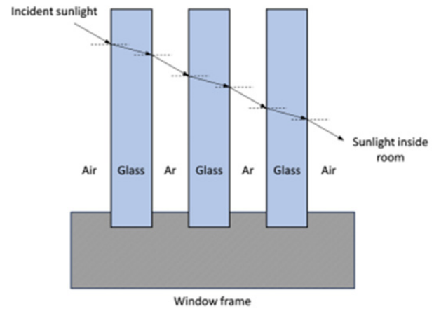
Figure 14. Illustration of light travel path at every interface in a triple glazing window having argon (Ar) in the window spacing. Sunlight travel paths at the interfaces are represented by the arrows. Modified figure from Ref. [28] .
