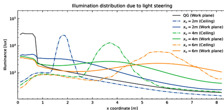
Figure 10. Illumination distribution due to light steering by our micromirror smart glass for a user position x_u = 2 m, 4 m and 6 m and by the reference glazing (QG) without micromirrors. Note that the work plane is 85 cm above the room floor. Modified figure from Ref. [28] .
