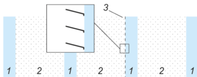
Figure 9. Glazing structure of the CFS with micromirrors (the left side faces the outside; the right side faces the inside of the room). Modified figure from Ref. [28] .
