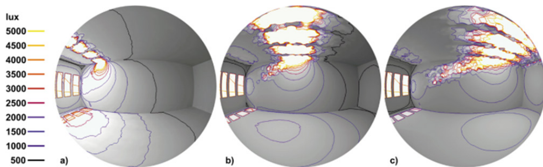
Figure 11. Rendered images in fish eye lens perspective from inside the model room to view the overall impression of the illumination distribution considering the generated light cones at x_u = 2 m (a), 4 m (b) and 6 m (c). Modified figure from Ref. [28] .
